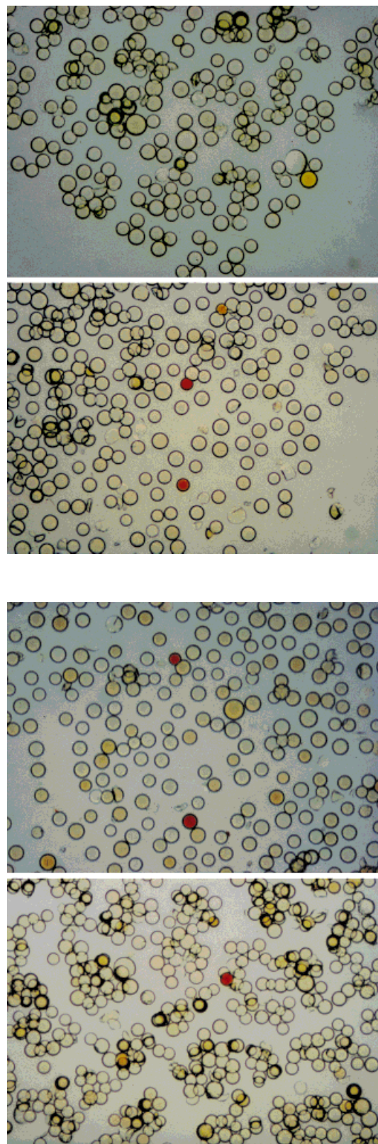
Figure 1. Photographs of the screening assays of tweezer receptors 1 , 2 , 3 , and 5 for binding to the bead-supported tripeptide library.
