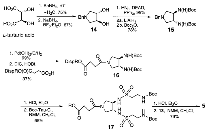
Scheme 3. Synthesis of the receptors 5 with the pyrrolidine hinge; Bn = benzyl, HOBT = 1-hydroxybenzotriazole, DEAD = diethylazodicarboxylate, R = Disperse Red.
