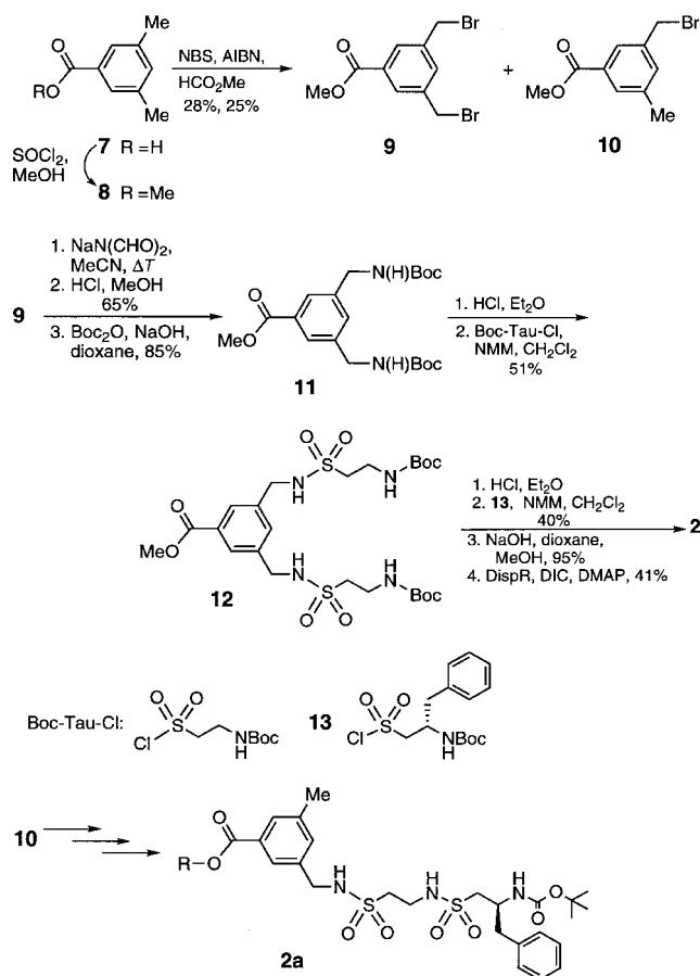
Scheme 2. Synthesis of the receptors 2 (with the bis(aminomethyl)benzoic acid hinge) and the amputated tweezer 2a ; NBS = N -bromosuccinimide, AIBN = azobisisobutyronitrile, Boc = tert -butoxycarbonyl, NMM = N -methylmorpholine, DIC = diisopropylcarbodiimide, DMAP = N,N -dimethylaminopyridine, R = Disperse Red.
